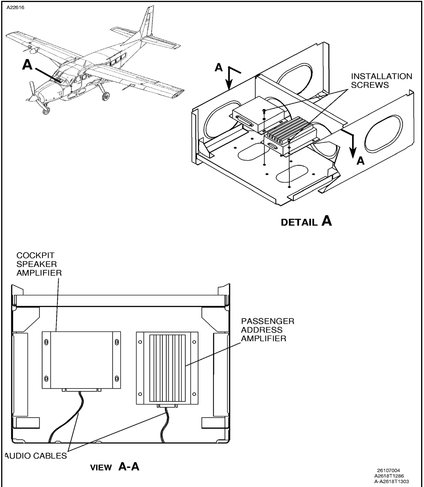
Figure 401 : Sheet 1 : Passenger Address and Cockpit Speaker Amplifier
